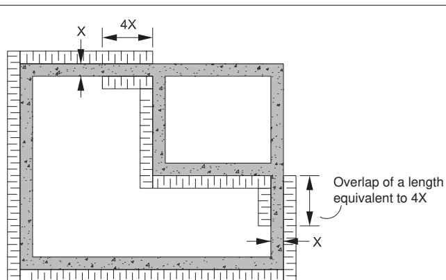
Figure A-3.2.1.2.(7)
