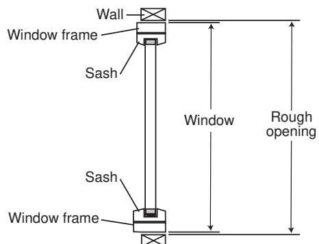
Figure A-3.1.1.6.(3)
