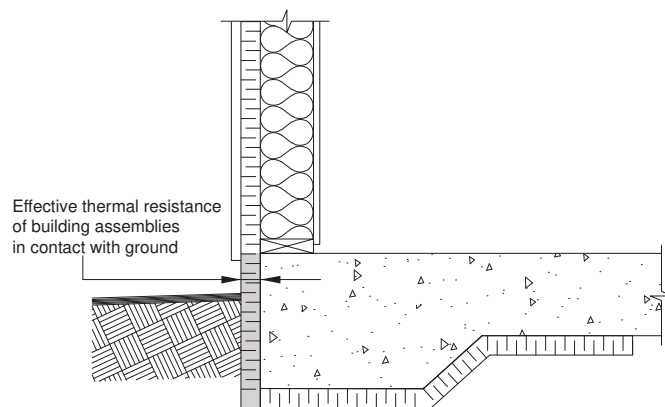
Figure A-3.2.3.1.(4)
