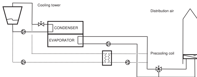
Figure A-5.2.2.9.-A
