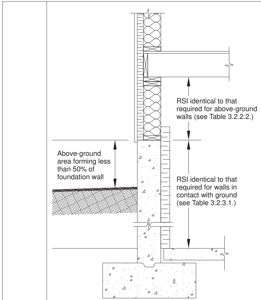
Figure A-3.2.2.2.(2) and (3)
