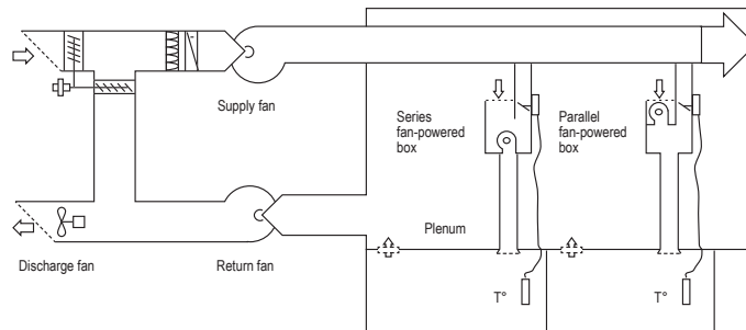
Figure A-5.2.3.1.(1), (2) and (3)
