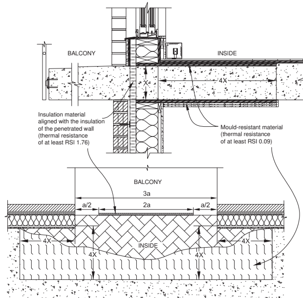
Figure A-3.2.1.2.(4)-C
