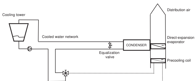
Figure A-5.2.2.9.-B
