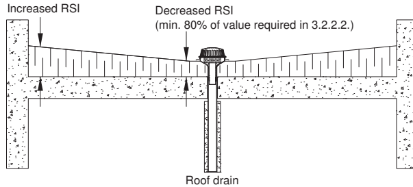
Figure A-3.2.2.2.(5) Reduction of the sloped insulation on a flat roof in accordance with Sentence 3.2.2.2.(5)
