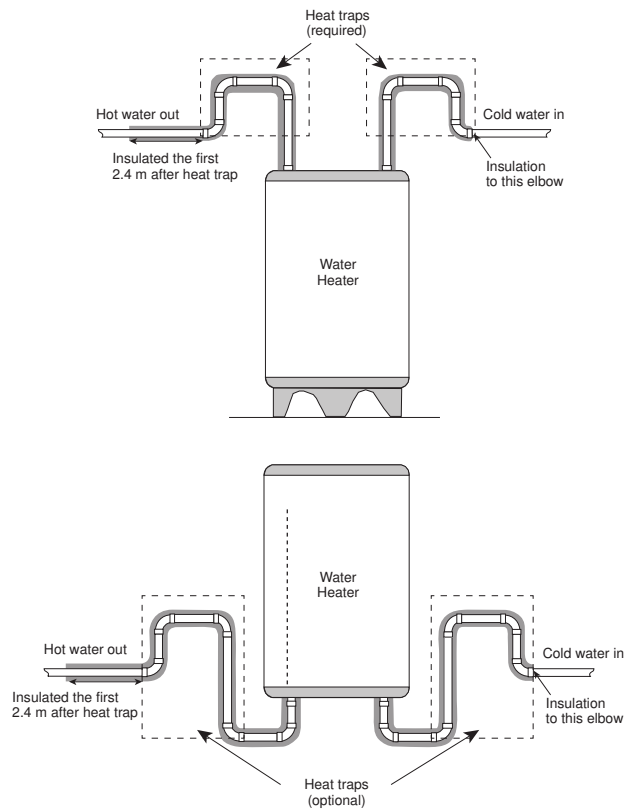
Figure A-6.2.3.1.(1) and (5) and 6.2.3.2.(1)
