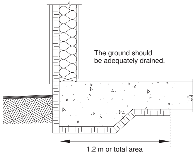
Figure A-3.2.3.3.-D Insulation of floors in contact with the ground for a slab-on-ground with integrated footings according to Sentence 3.2.3.3.(3)”. The ground should be adequately drained. 1.2 m or total area
